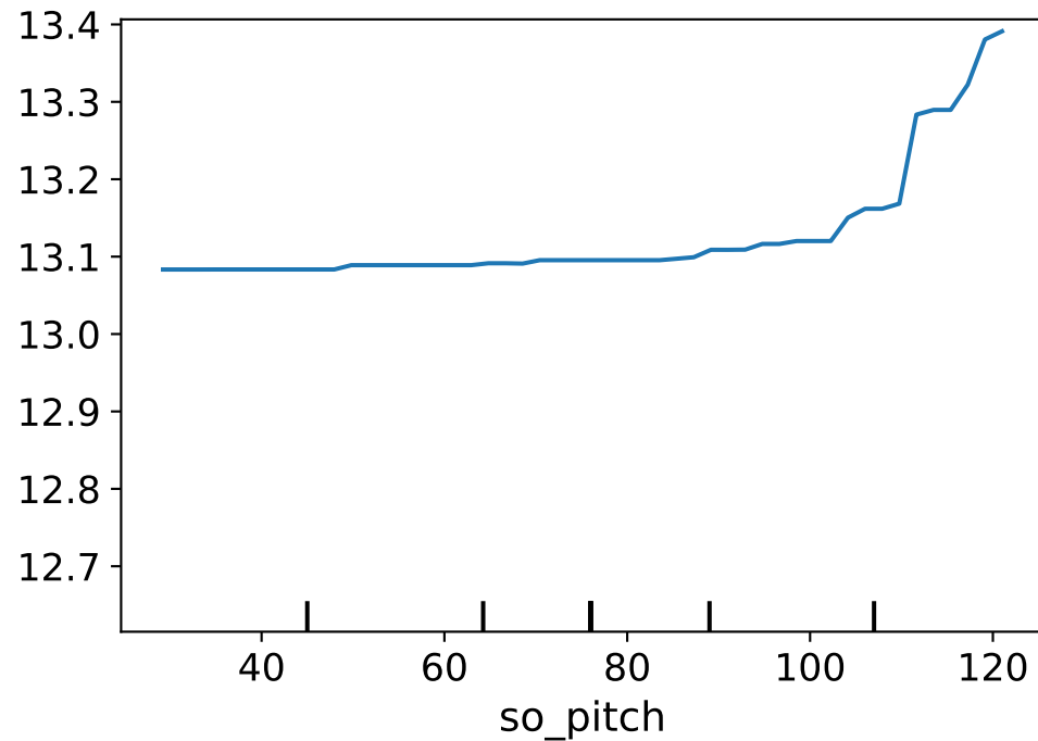
Stage 3: Slot Value: Partial Dependence
